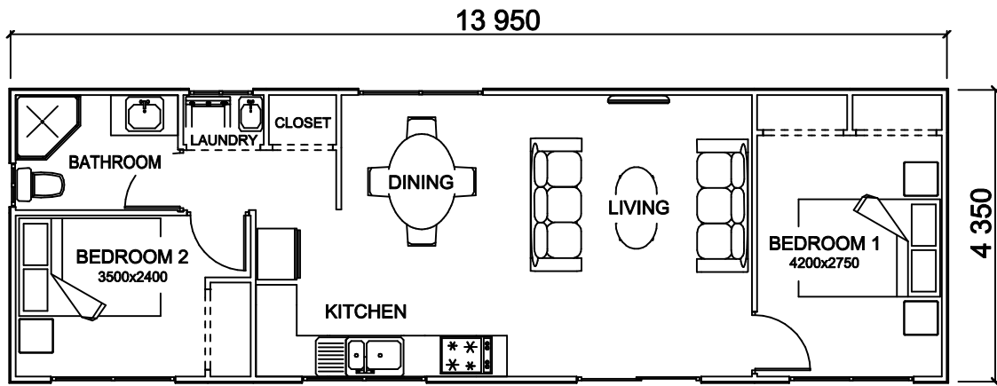
FLOOR PLAN
